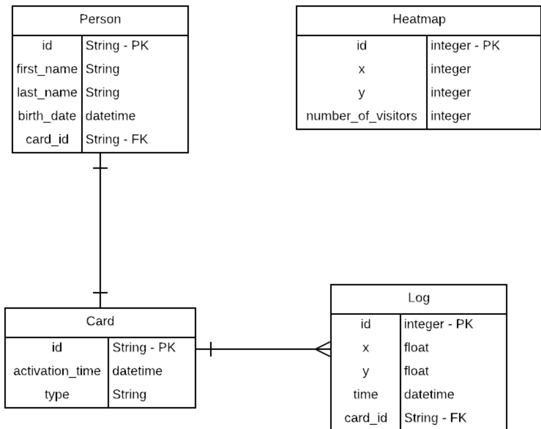
Figure 4: IPS Database ER Diagram
